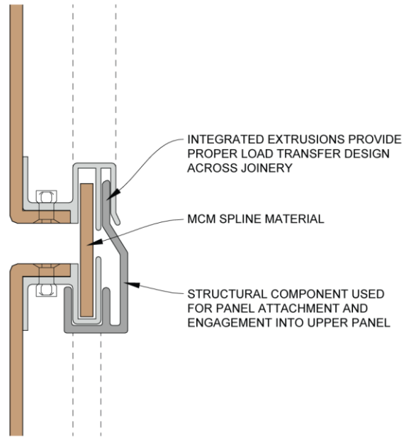
Figure 4- Spline System Horizontal Joint (Example)
